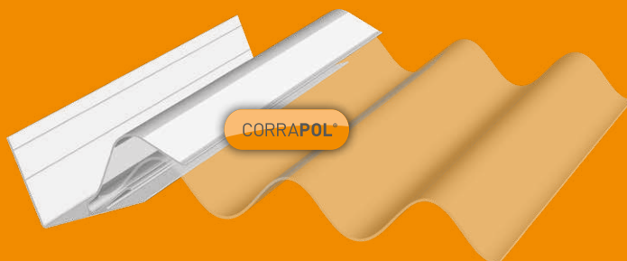
b Tilt the Corrapol® Rock N Lock® Wall Flashing to the side and fit the first corrugated sheet peak into the flashing.
