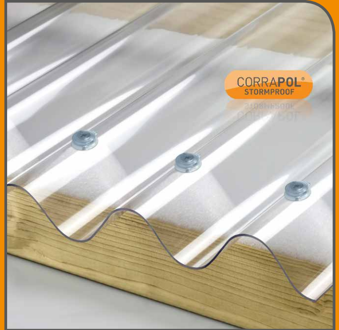
Corrapol® Stormproof® high profile in-situ view
