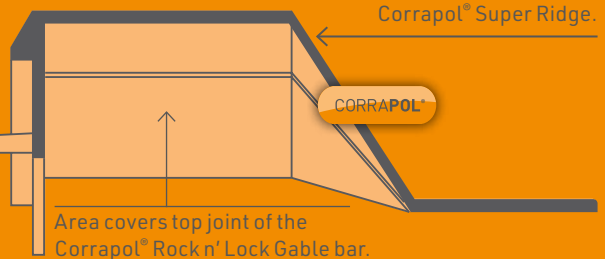
Cross Section of Corrapol® Super Ridge End Cap
